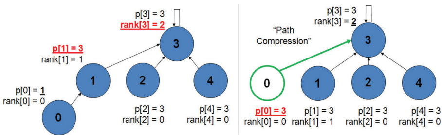
Рис. 2.7 ❖ unionSet(0, 3) → findSet(0)
